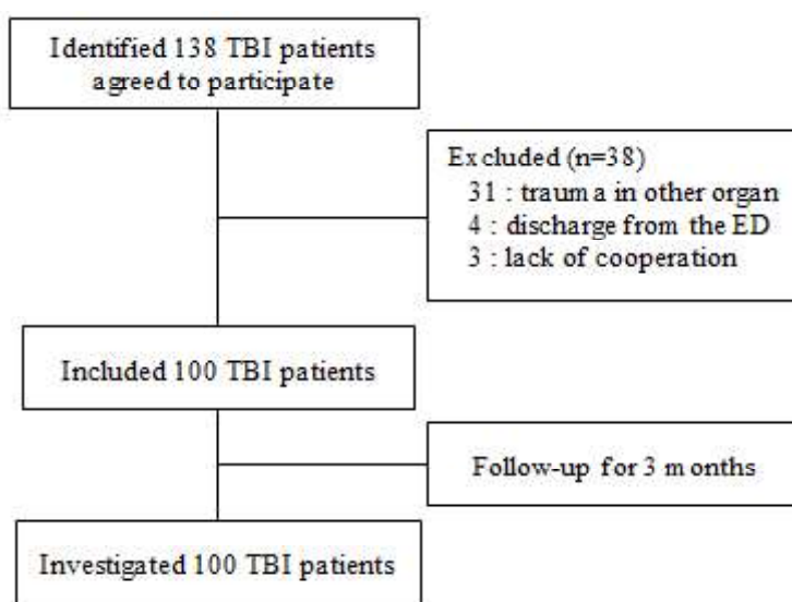
Figure 1. Flow diagram of traumatic brain injury
